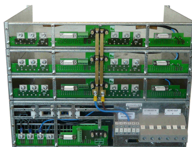
Rear panel 9kVA system with static switch/manual bypass 3 x MSR8170 powerframe for 6 x inverters, MBP68400 for 30kVA static switch and manual bypass
